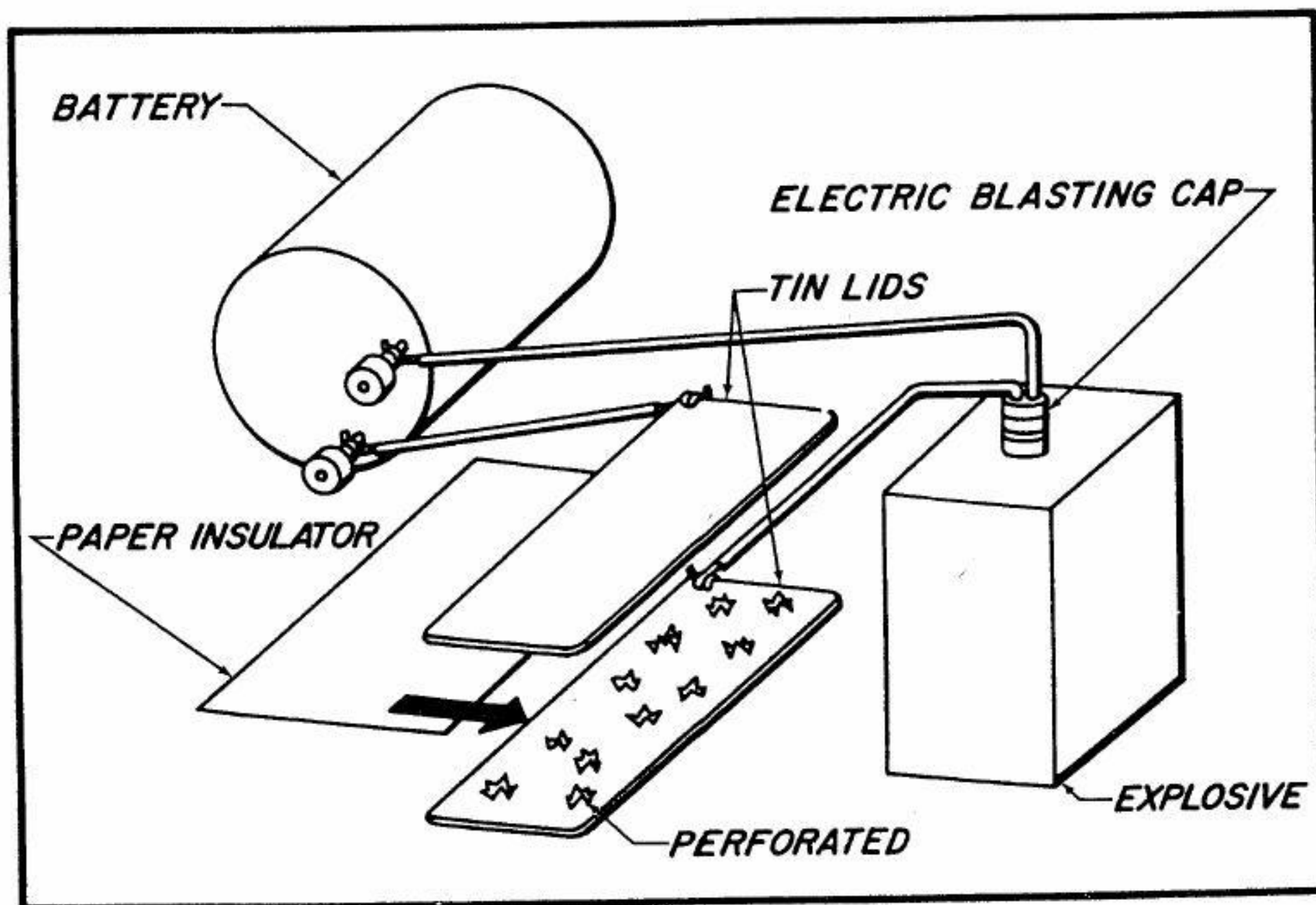
Fig. 6 — Electric Pressure Switch (Lids)
