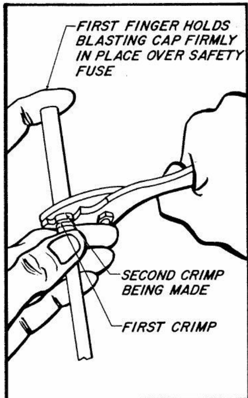
Fig. 1 — Crimping
