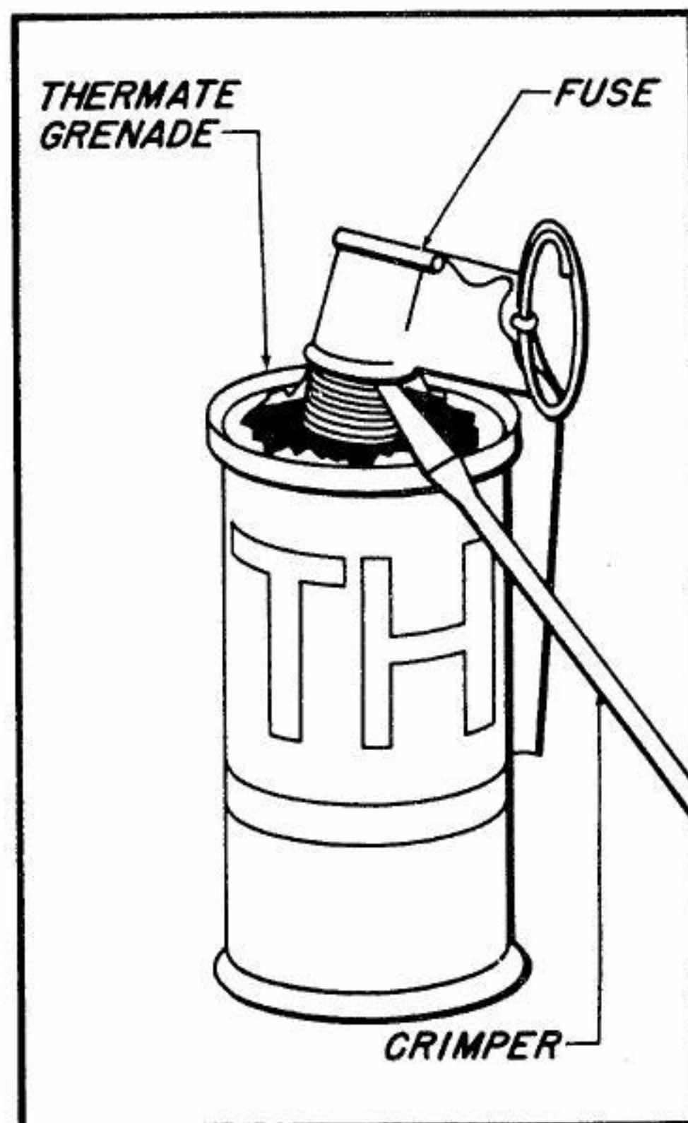
Fig. 61 — Defusing Thermate Grenade
