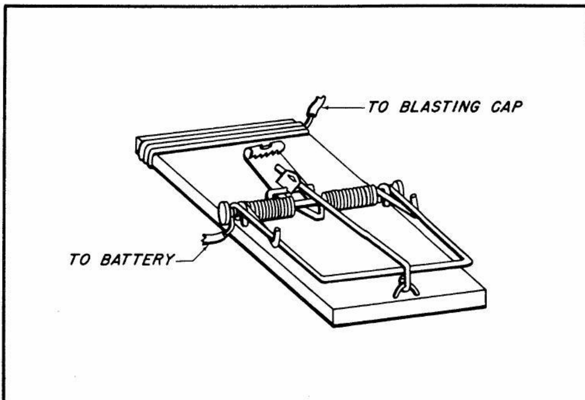
Fig. 14 — Mousetrap Electric Release
