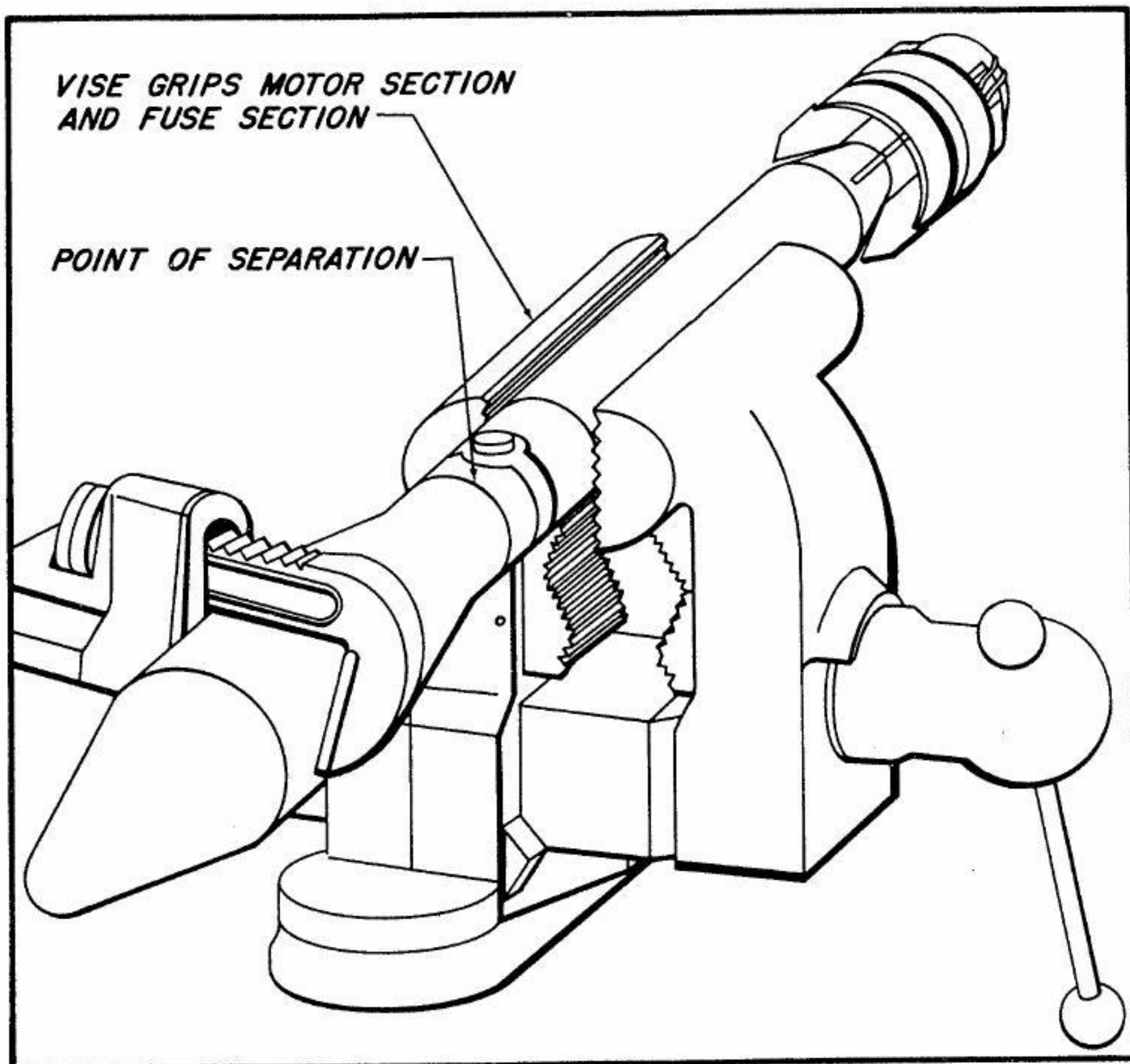
Fig. 52 — Removing Rocket Head
