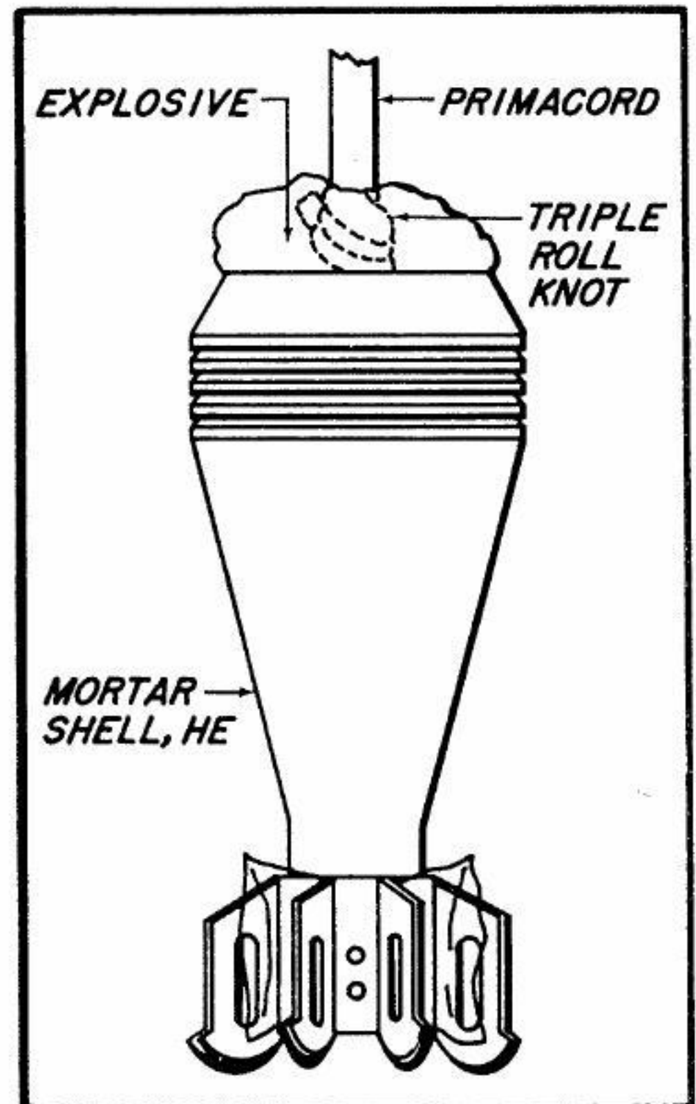
Fig. 49 — Priming Mortar Shell
