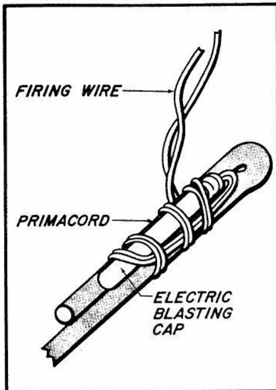
Fig. 3 — Electric Cap and Primacord
