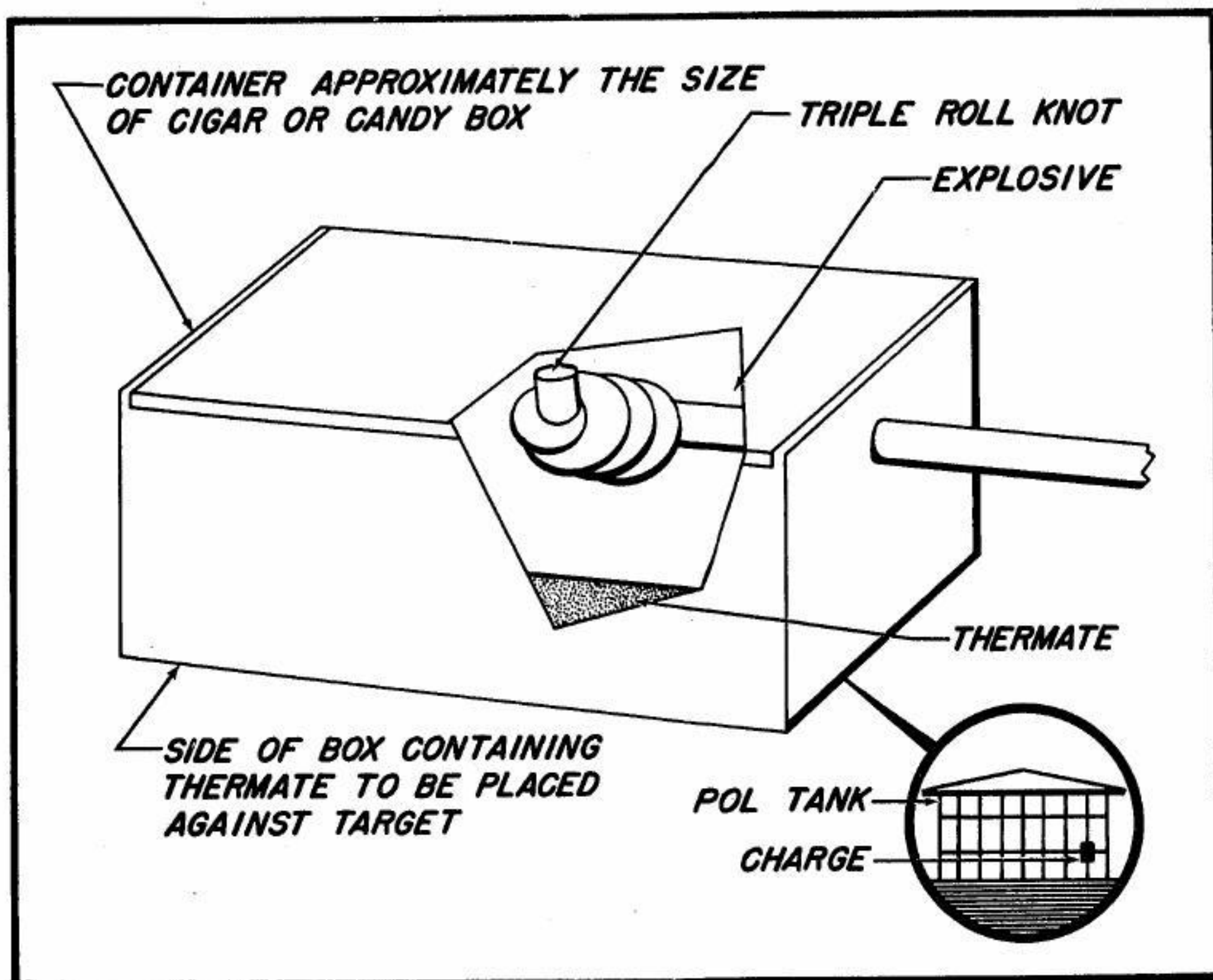
Fig. 65 — Cigar Box Charge
