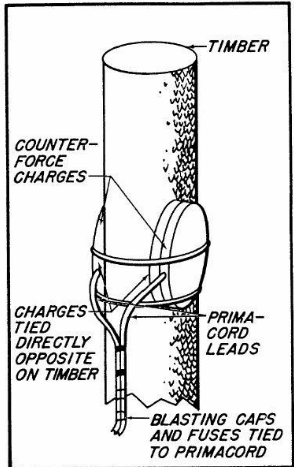
Fig. 41 — Counterforce Charge Placement
