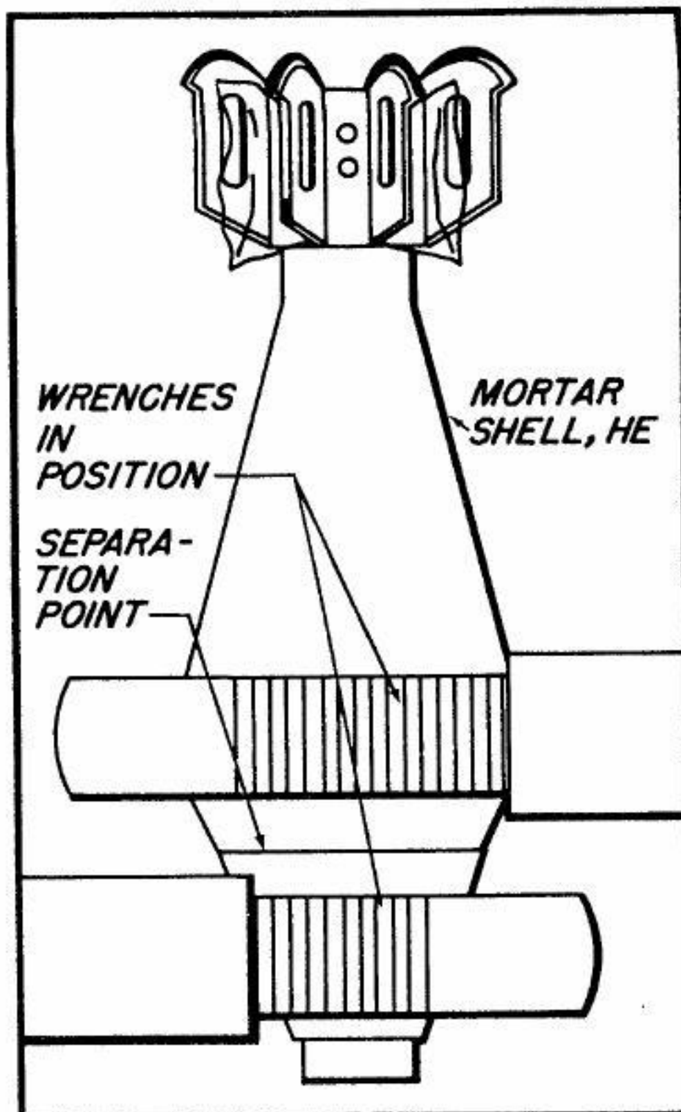
Fig. 48 — Removing Mortar Shell Fuse
