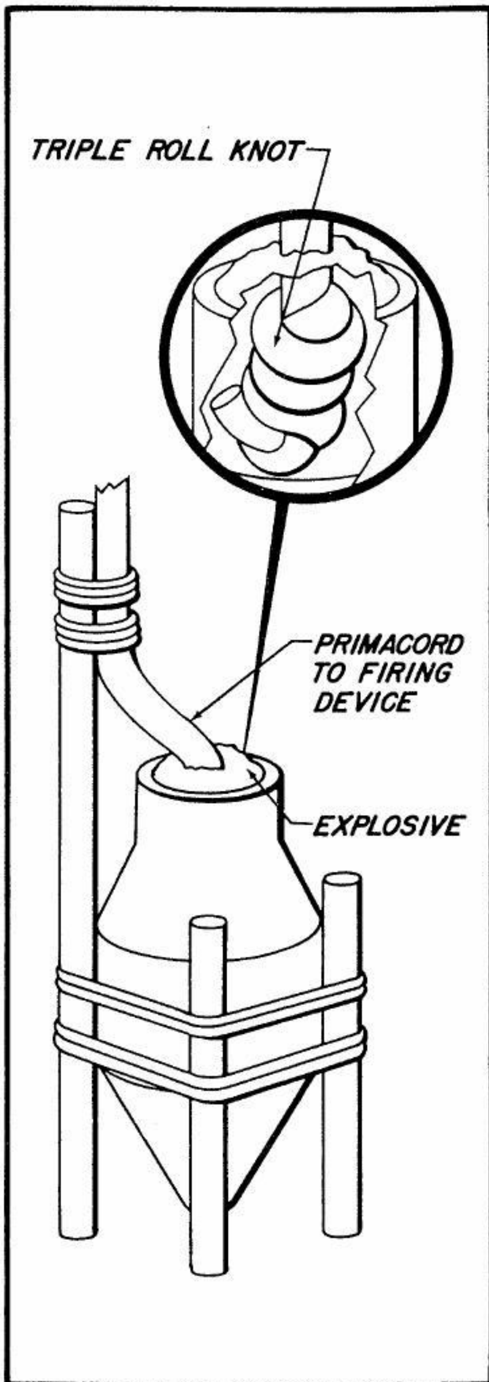
Fig. 53 — Rocket Shaped Charge
