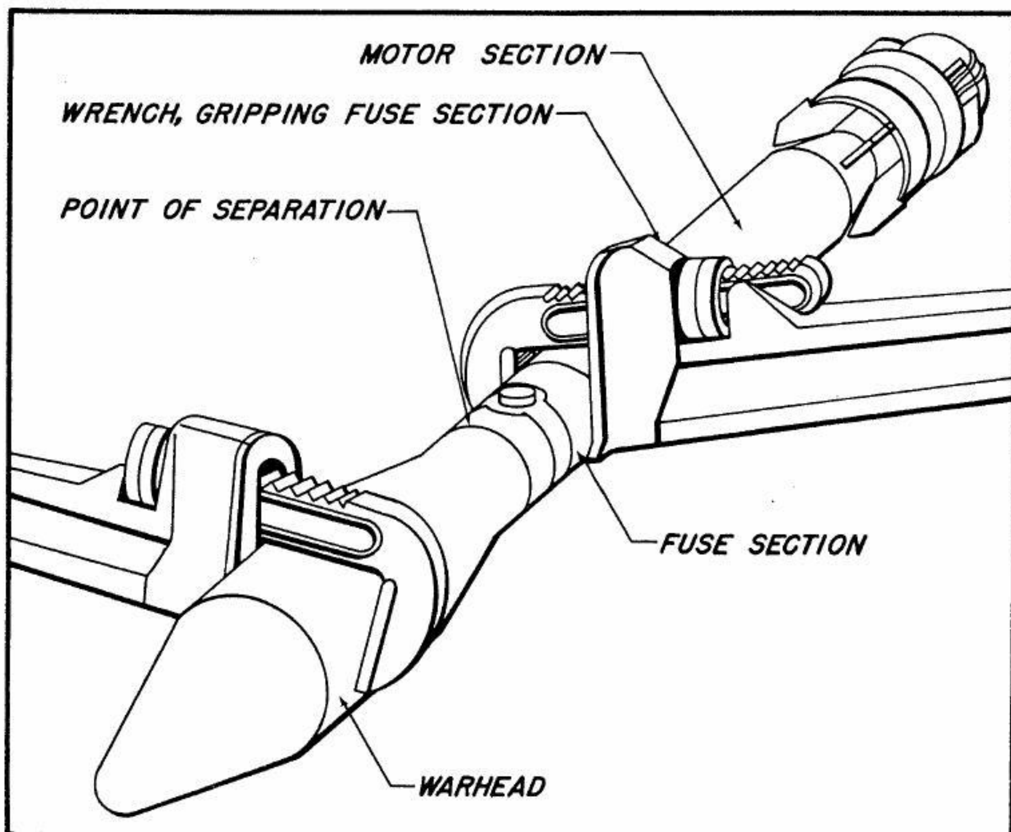
Fig. 51 — Removing Rocket Head
