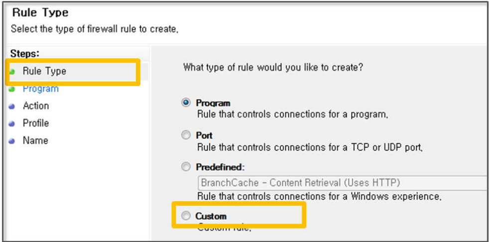
Figure 2-36 Rule Type
