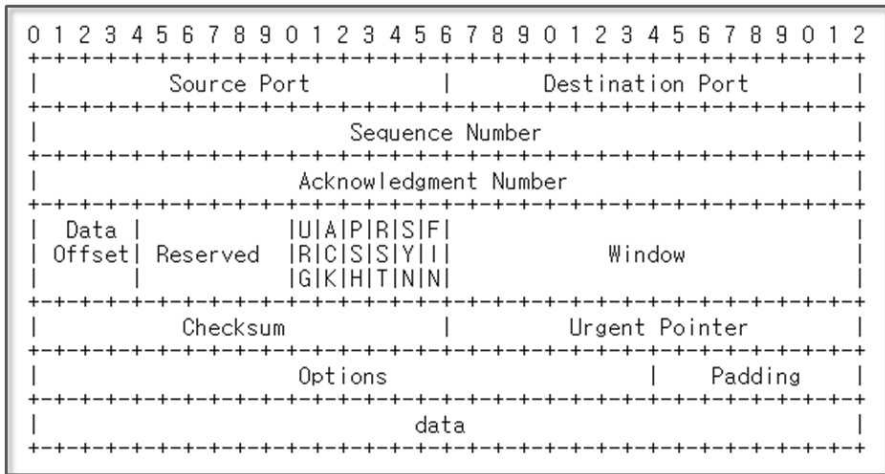
Figure 2-61 TCP Header
