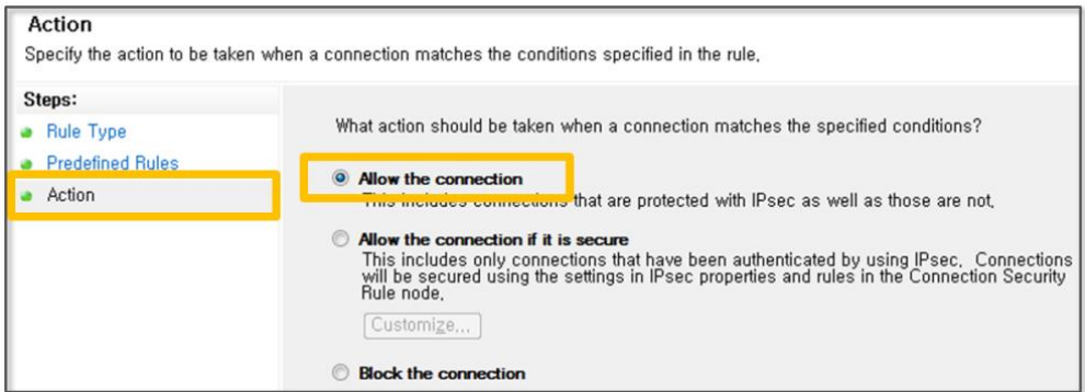
Figure 2-15 Select Action
