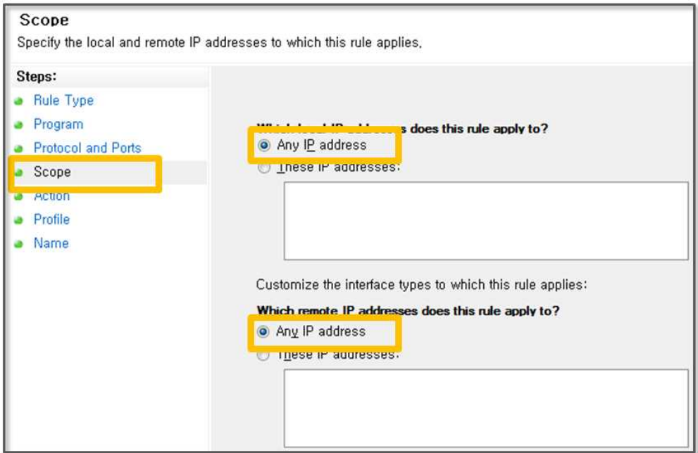
Figure 2-40 Select Scope
