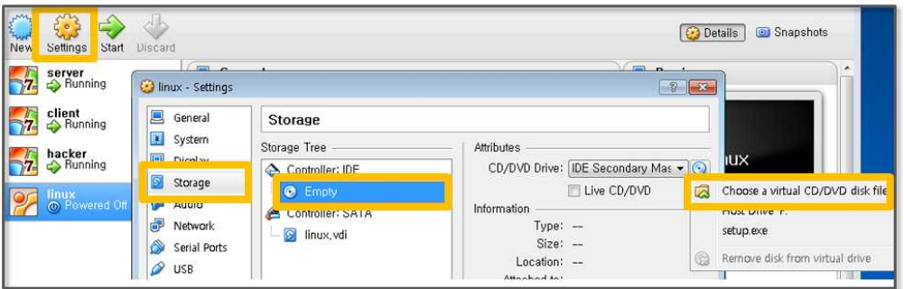
Figure 2-51 Select Installer
