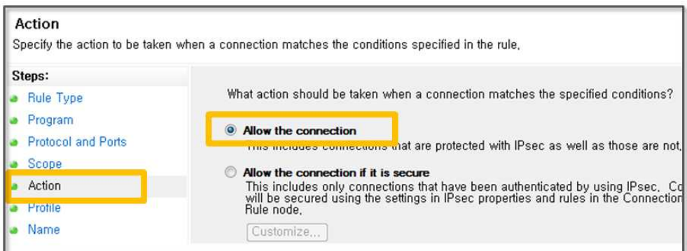
Figure 2-41 Select Action
