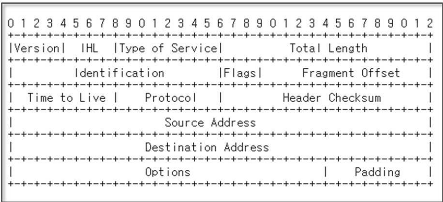
Figure 2-59 IP Header
