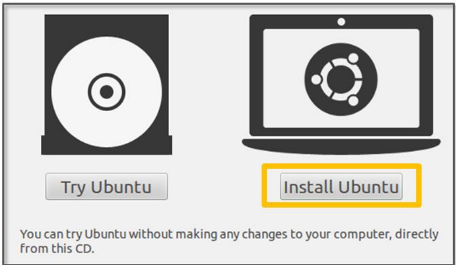
Figure 2-53 Linux Install
