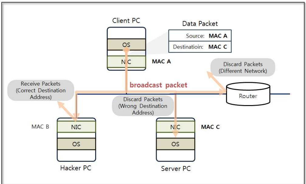
Figure 2-28 TCP / IP Layer-2 Protocol behavior
