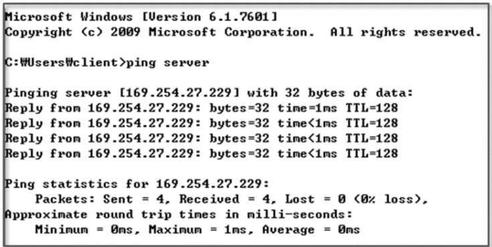
Figure 2-43 Check Setting
