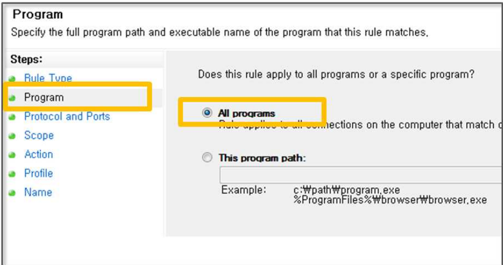
Figure 2-37 Programs
