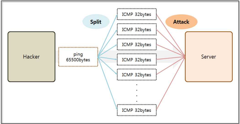
Figure 2-44 Concept of the Ping of Death
