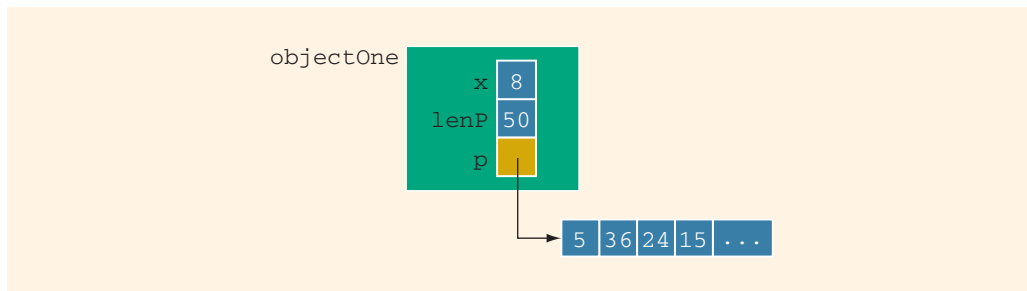
FIGURE 14-14 Object objectOne and its data
