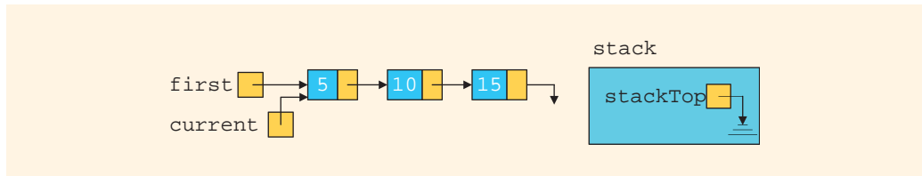
FIGURE 19-25 List and stack after the statements current = stack.top(); and stack.pop(); execute
