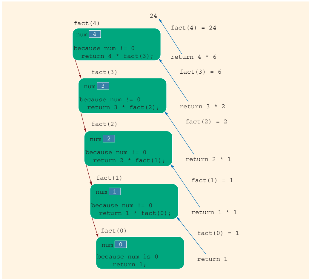
FIGURE 17-1 Execution of fact(4)
