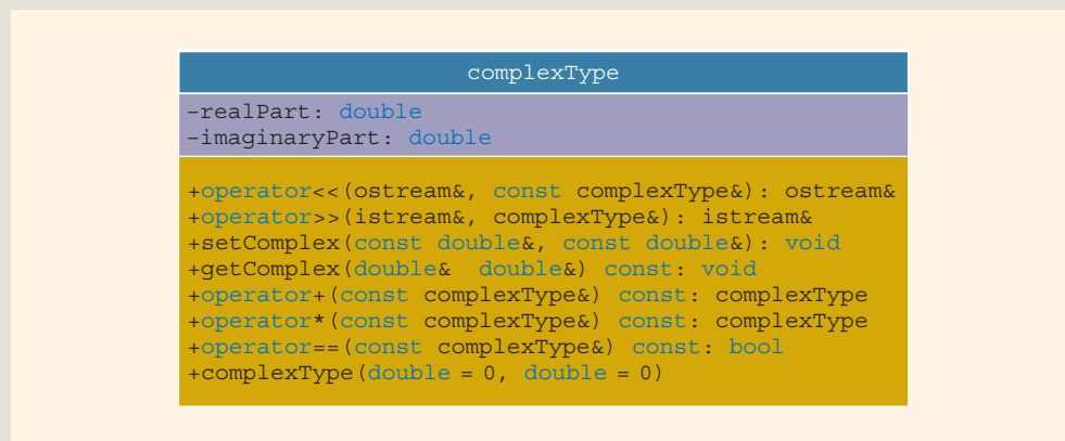
FIGURE 15-2 UML class diagram of the class complexType
