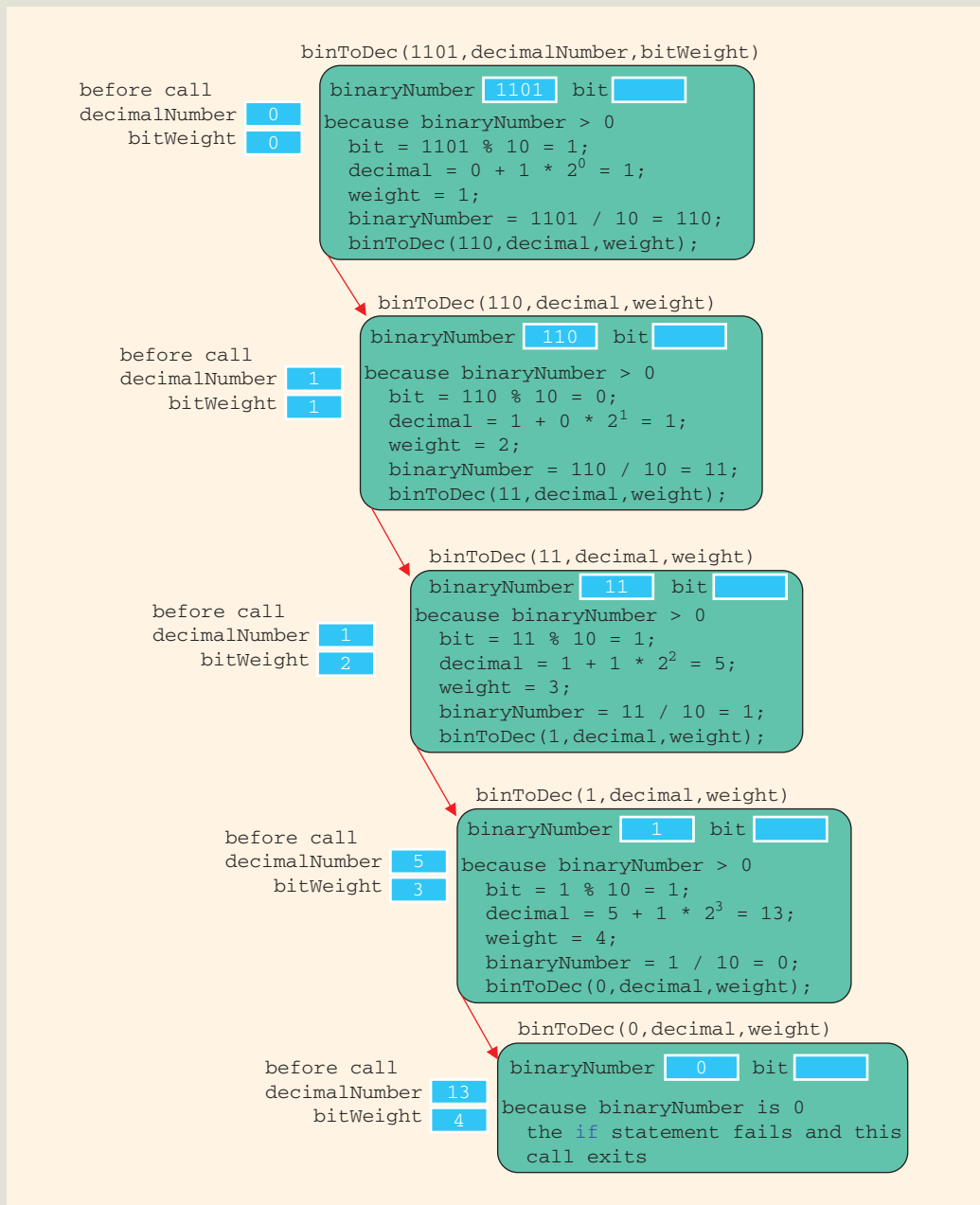
FIGURE 17-8 Execution of binToDec(1101, decimalNumber, bitWeight);
