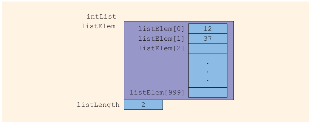
FIGURE 11-6 intList after the statements in Lines 1 through 5 execute
