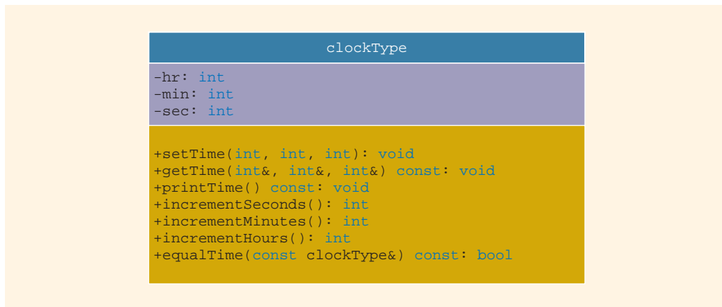
FIGURE 12-1 UML class diagram of the clockType class
