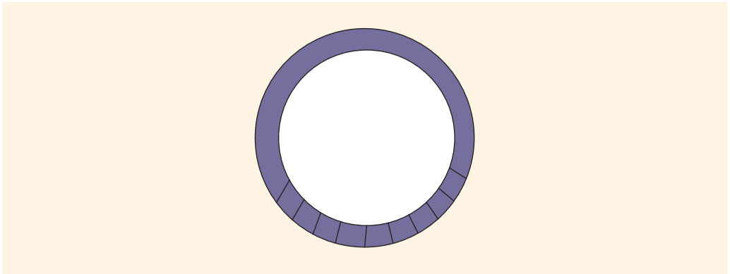
FIGURE 19-30 Circular queue
