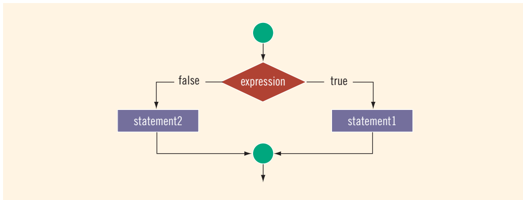
FIGURE 4-3 Two-way selection
