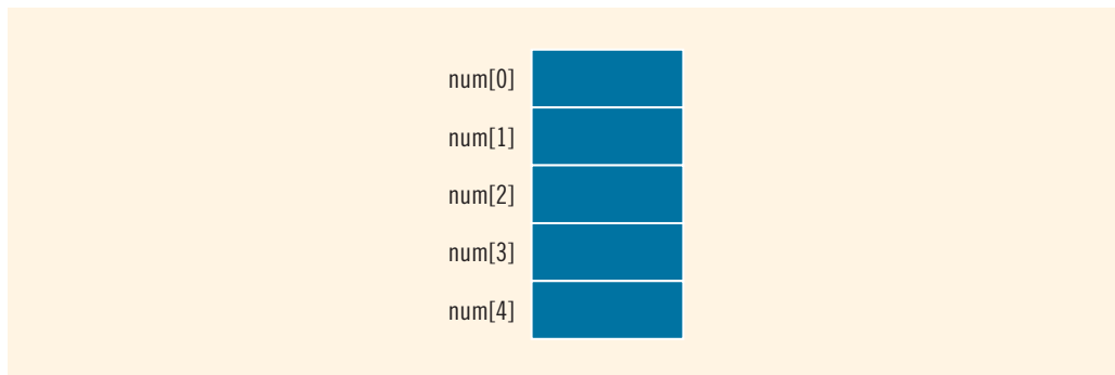
FIGURE 9-1 Array num
