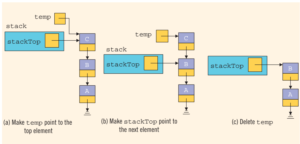
FIGURE 19-16 Pop operation
