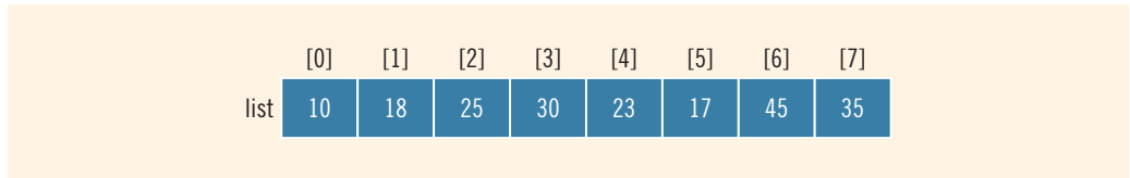
FIGURE 10-9 list
