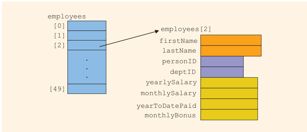
FIGURE 11-7 Array of employees
