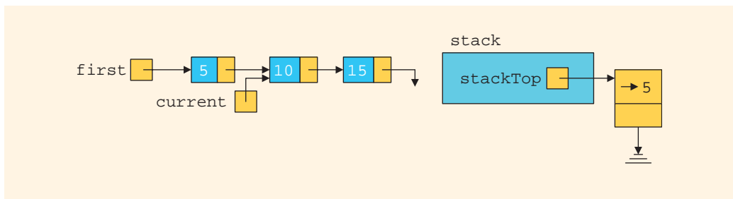
FIGURE 19-24 List and stack after the statements current = stack.top(); and stack.pop(); execute
