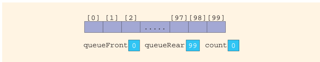
FIGURE 19-35 Empty queue
