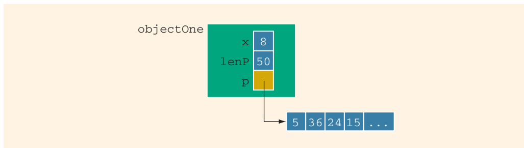
FIGURE 14-19 Object objectOne
