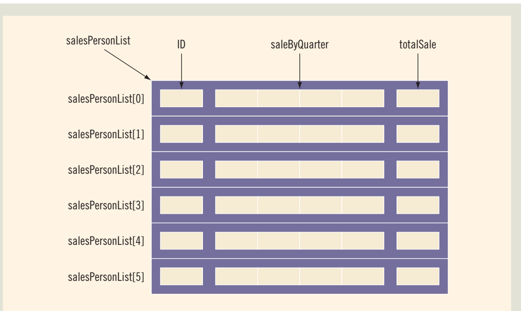
FIGURE 11-9 Array salesPersonList
