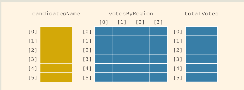
FIGURE 10-20 Parallel arrays: candidatesName , votesByRegion , and totalVotes
