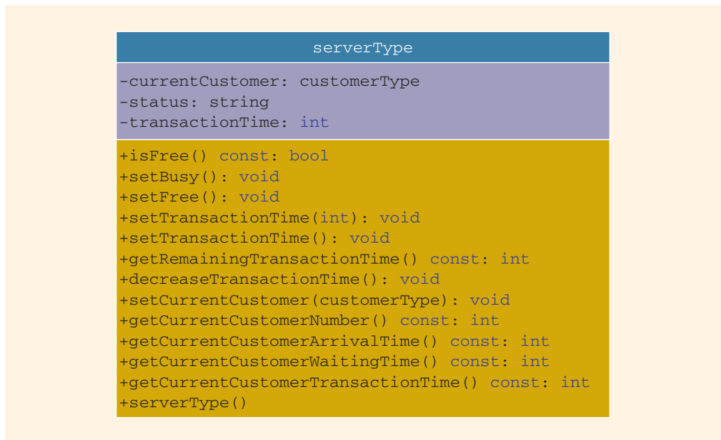
FIGURE 19-37 UML class diagram of the class serverType
