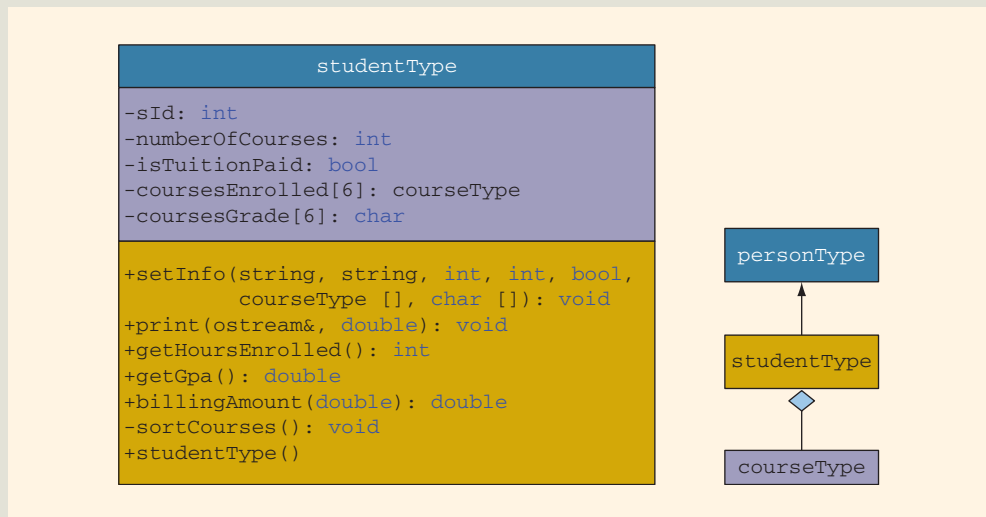
FIGURE 13-10 UML class diagram of the class studentType together with inheritance and composition (aggregation) relation
