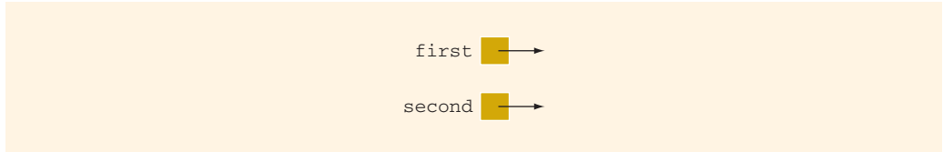
FIGURE 14-11 first and second after the statement delete [] second; executes
