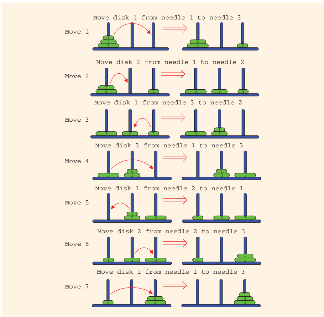
FIGURE 17-7 Solution to Tower of Hanoi problem with three disks
