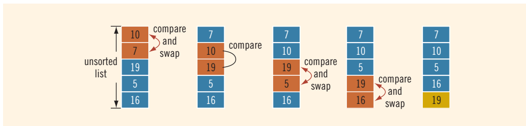
FIGURE 10-2 Elements of list during the first iteration
