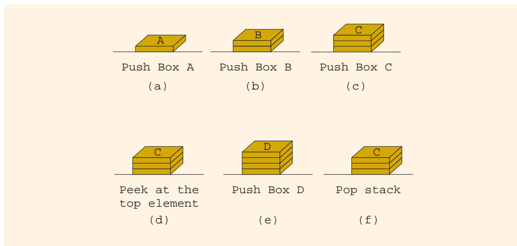
FIGURE 19-3 Stack operations
