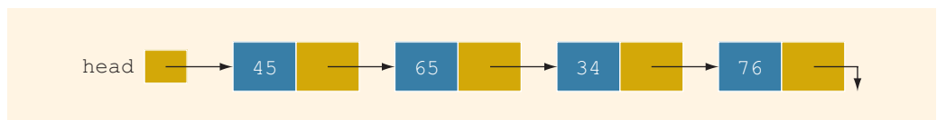
FIGURE 18-2 Linked list
