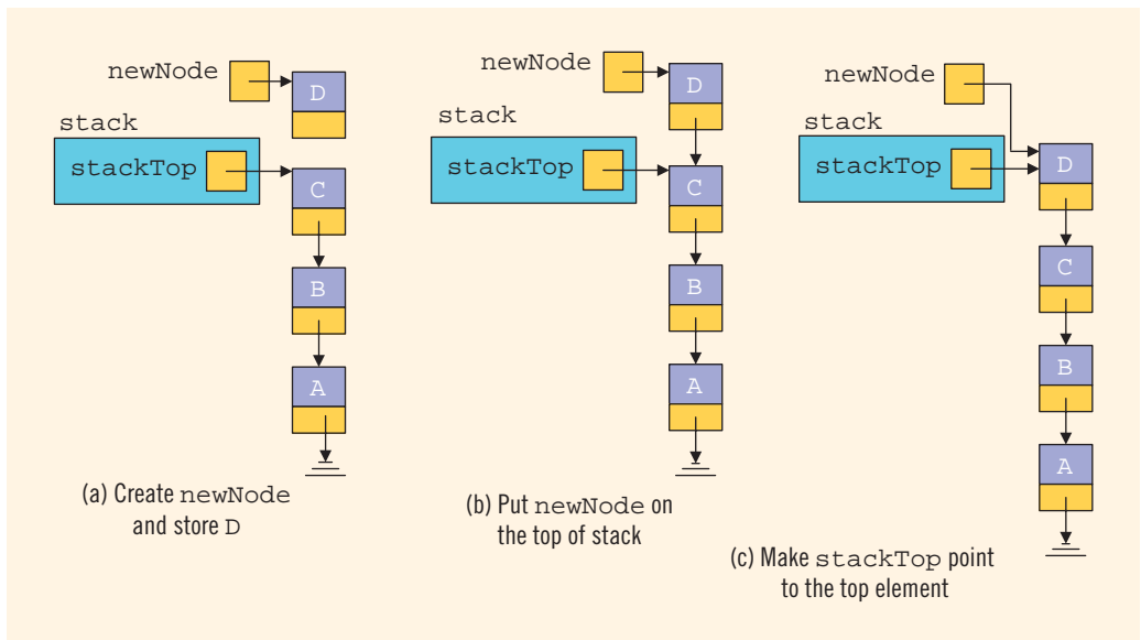
FIGURE 19-14 Push operation
