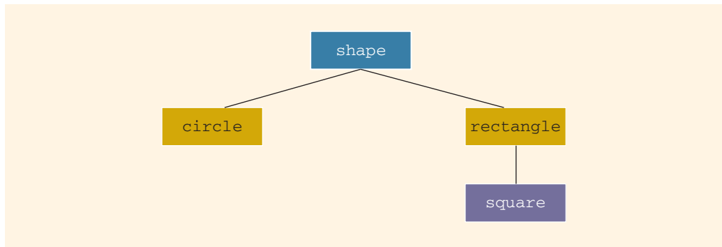
FIGURE 13-1 Inheritance hierarchy
