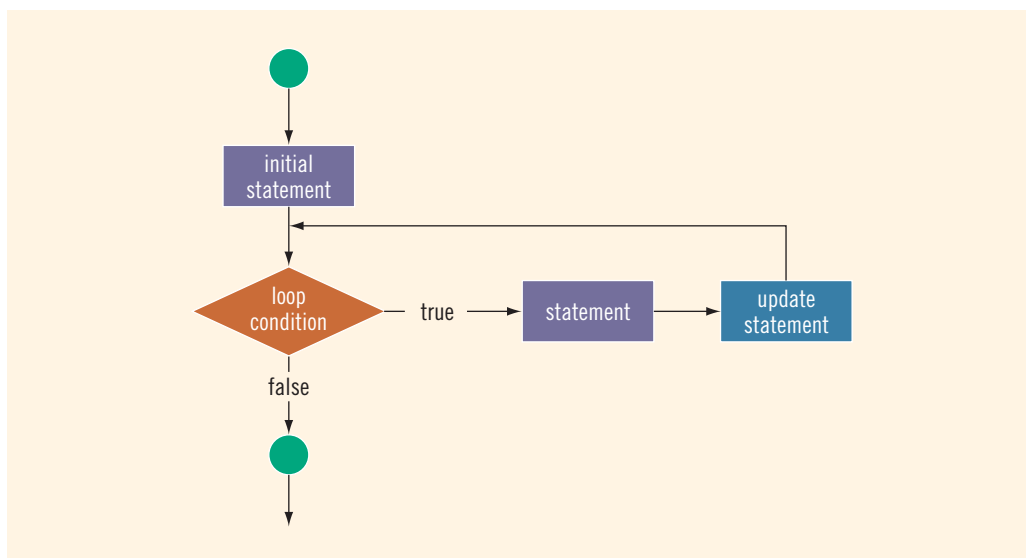
FIGURE 5-2 for loop
