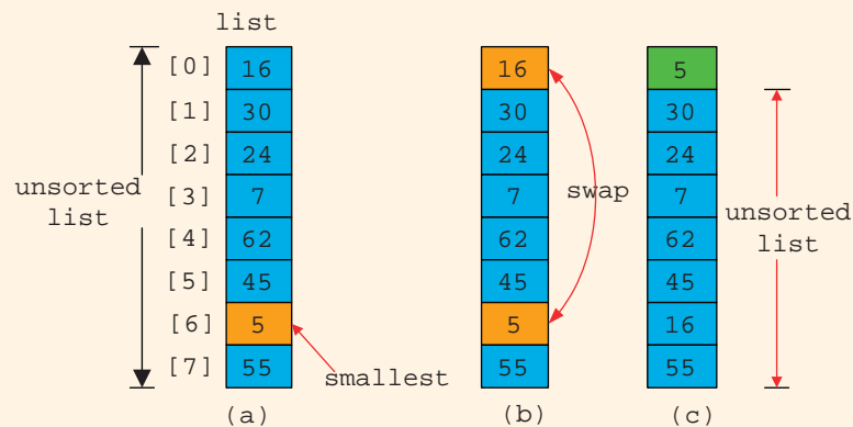
FIGURE 10-7 Elements of list during the first iteration
