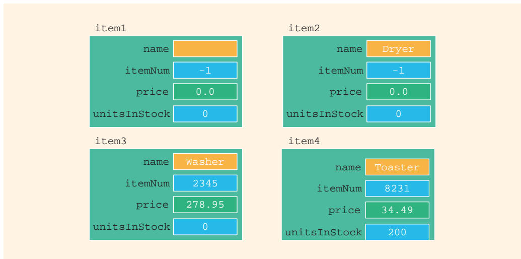
FIGURE 12-7 Effect of constructors on objects
