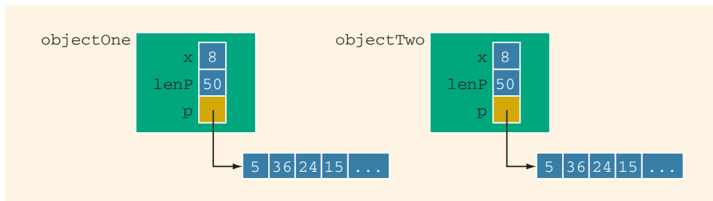
FIGURE 14-17 Objects objectOne and objectTwo
