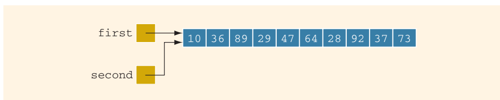
FIGURE 14-10 first and second after the statement second = first; executes
