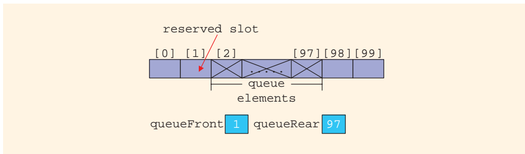
FIGURE 19-34 Array to store the queue elements with a reserved slot
