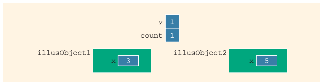
FIGURE 12-13 illusObject1 and illusObject2 after the statements illustrate::incrementY(); and illustrate::count++; execute
