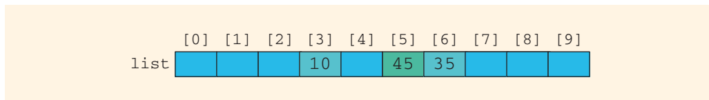
FIGURE 9-5 Array list after execution of the statements list[3]= 10; , list[6]= 35; , and list[5] = list[3] + list[6];
