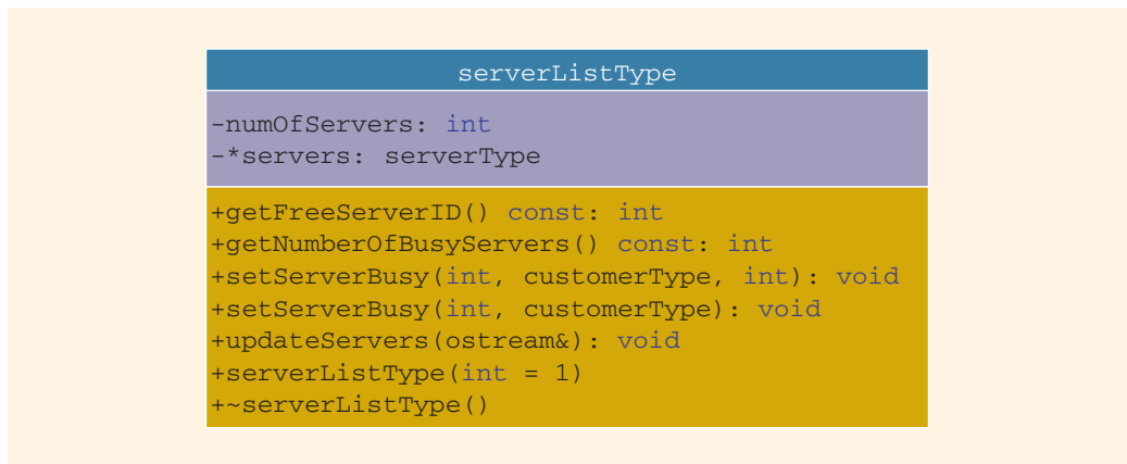
FIGURE 19-38 UML class diagram of the class serverListType
