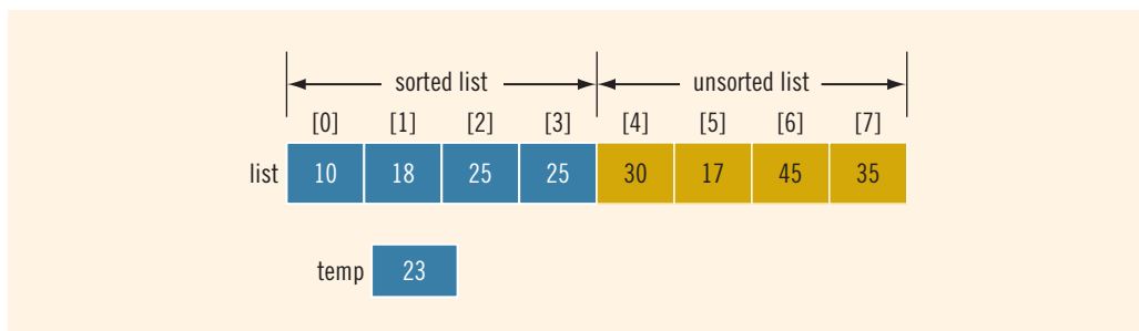
FIGURE 10-14 list after copying list[3] into list[4] and then list[2] into list[3]
