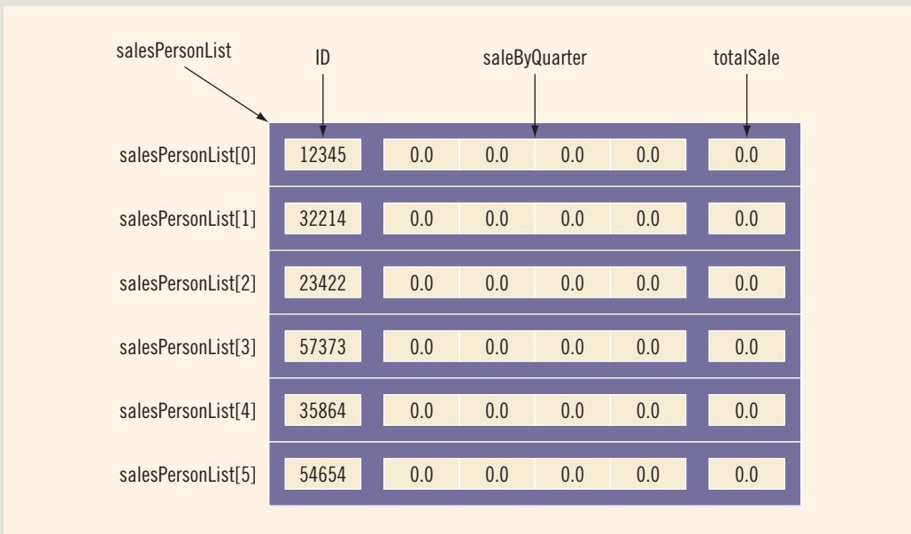
FIGURE 11-10 Array salesPersonList after initialization
