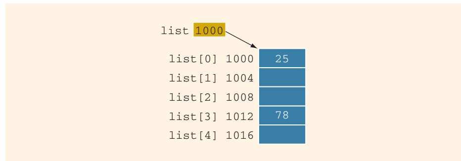
FIGURE 14-7 Array list after the execution of the statements list[0] = 25; and list[3] = 78;
