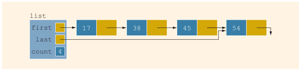
FIGURE 18-35 list before inserting 27
