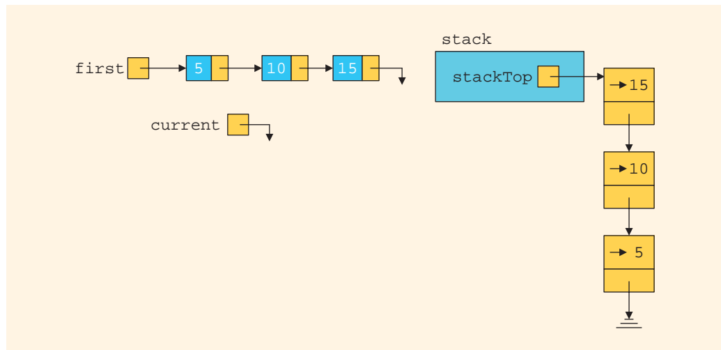
FIGURE 19-22 List and stack after the statements stack.push(current); and current = current->link; execute
