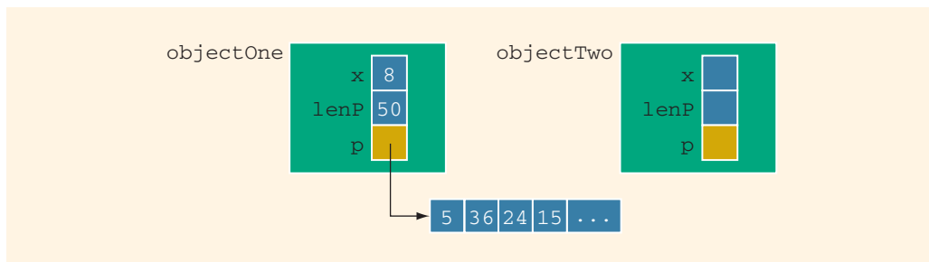
FIGURE 14-15 Objects objectOne and objectTwo
