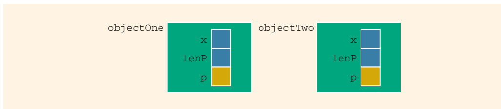
FIGURE 14-13 Objects objectOne and objectTwo
