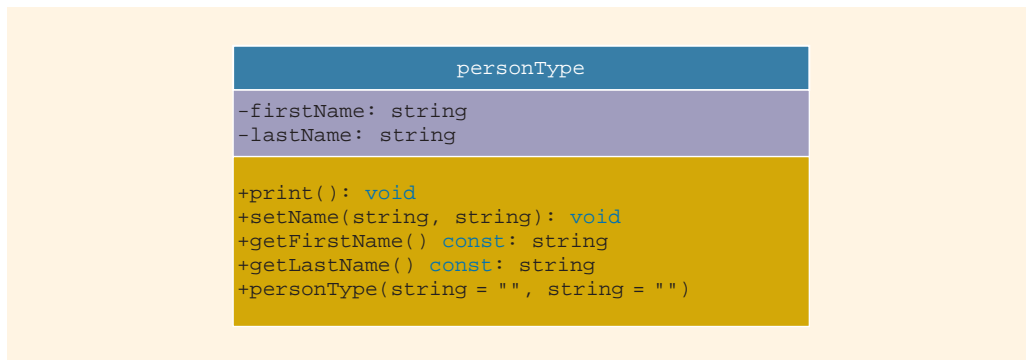
FIGURE 12-11 UML class diagram of the class personType
