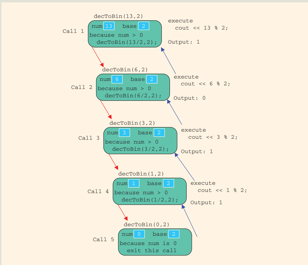
FIGURE 17-9 Execution of decToBin(13, 2)
