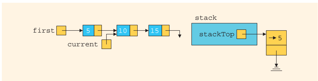
FIGURE 19-20 List and stack after the statements stack.push(current); and current = current->link; execute
