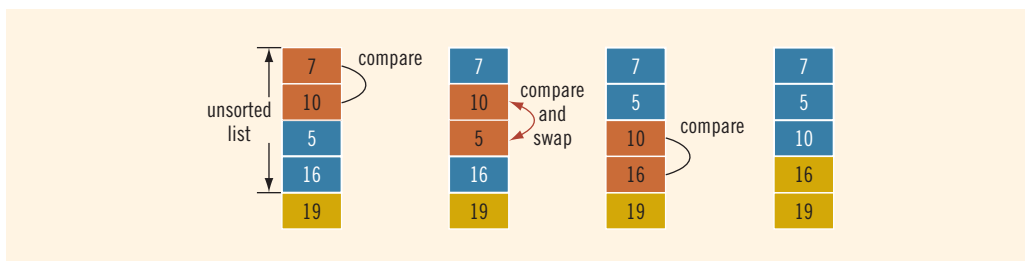
FIGURE 10-3 Elements of list during the second iteration
