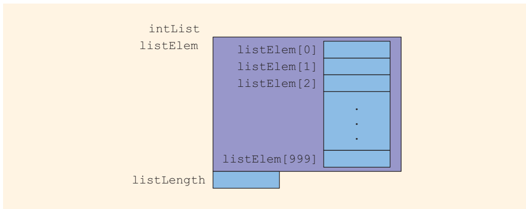
FIGURE 11-5 struct variable intList
