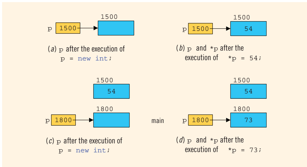
FIGURE 14-5 p after the memory space it points to following the execution of various statements
