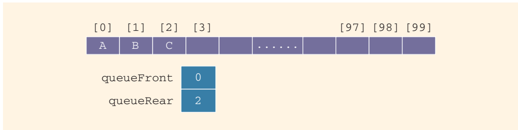
FIGURE 19-27 Queue after two more addQueue operations
