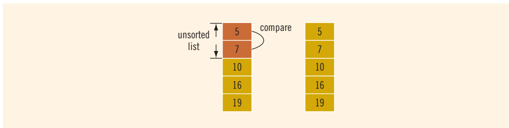
FIGURE 10-5 Elements of list during the fourth iteration
