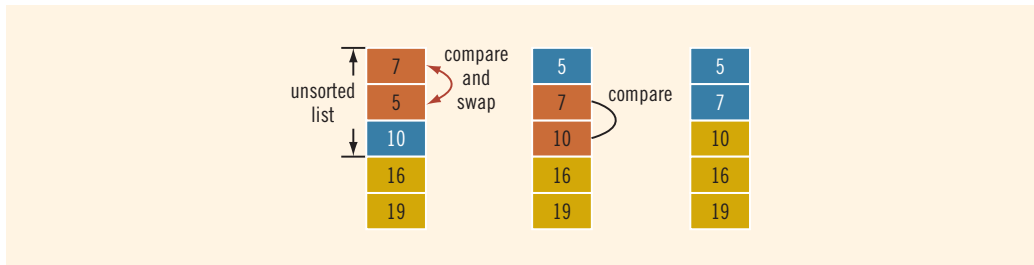
FIGURE 10-4 Elements of list during the third iteration
