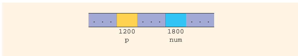
FIGURE 14-1 Variables p and num
