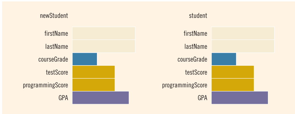
FIGURE 11-1 structs newStudent and student
