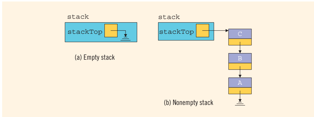
FIGURE 19-12 Empty and nonempty linked stack
