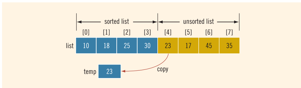
FIGURE 10-12 Copy list[4] into temp
