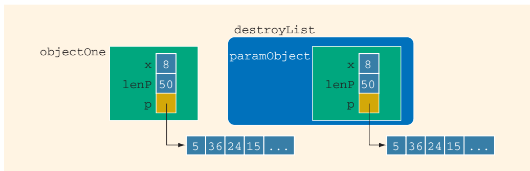
FIGURE 14-21 Pointer member variables of objects objectOne and paramObject with their own data
