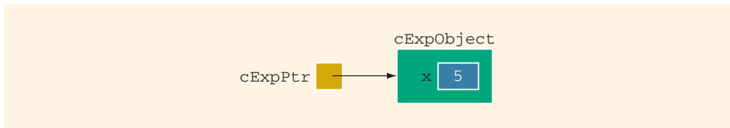
FIGURE 14-4 cExpObject and cExpPtr after the statement cExpPtr->setX(5); executes
