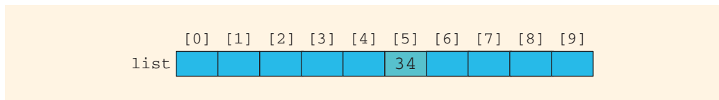
FIGURE 9-4 Array list after execution of the statement list[5]= 34;
