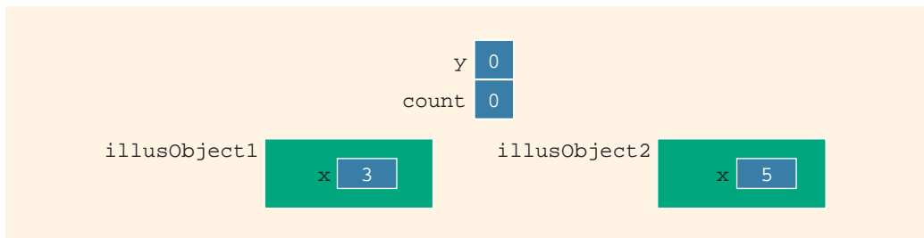
FIGURE 12-12 illusObject1 and illusObject2
