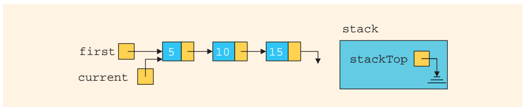
FIGURE 19-19 List after the statement current = first; executes
