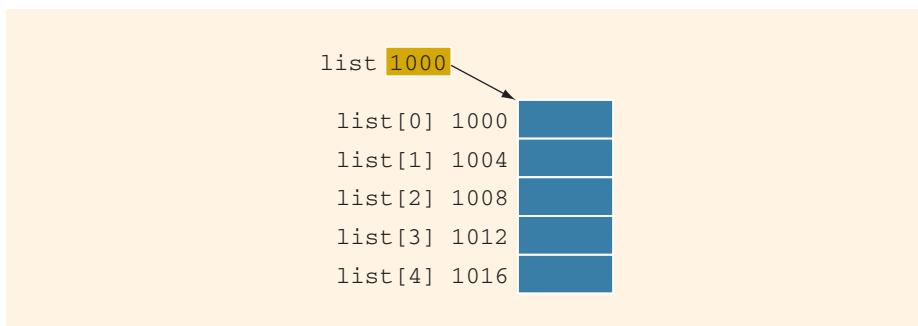
FIGURE 14-6 list and array list
