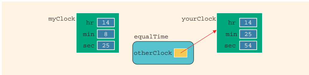
FIGURE 12-6 Object myClock and parameter otherClock
