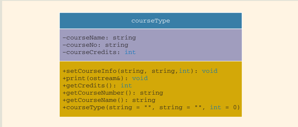
FIGURE 13-9 UML class diagram of the class courseType
