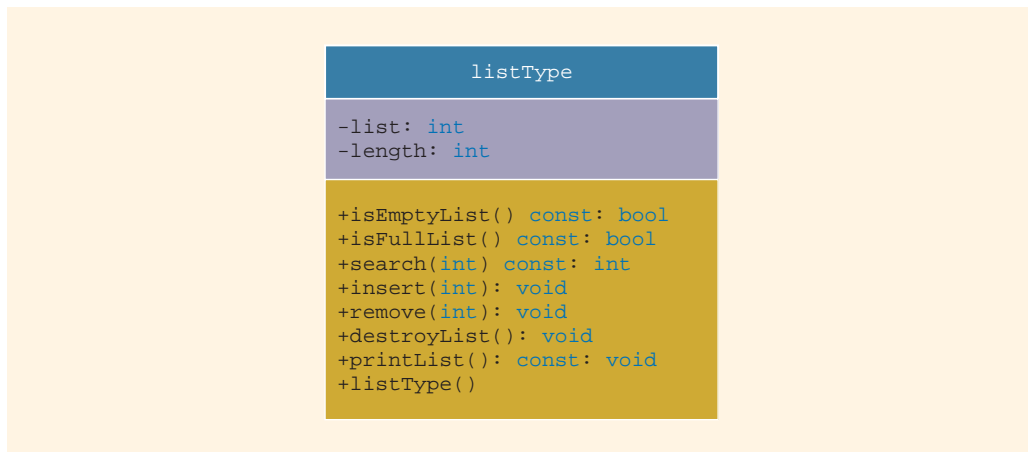
FIGURE 12-10 UML class diagram of the class listType
