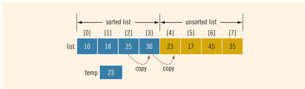
FIGURE 10-13 list before copying list[3] into list[4] and then list[2] into list[3]
