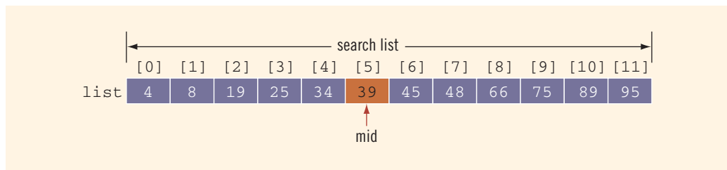
FIGURE 10-17 Search list, list[0]...list[11]
