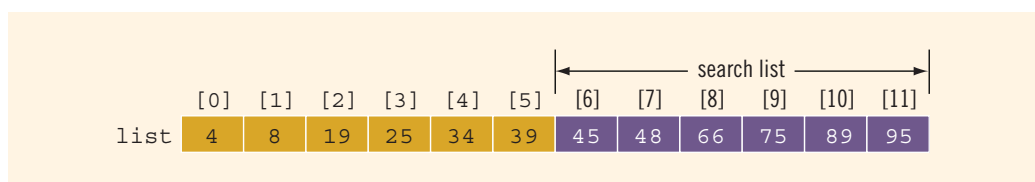
FIGURE 10-18 Search list, list[6]...list[11]
