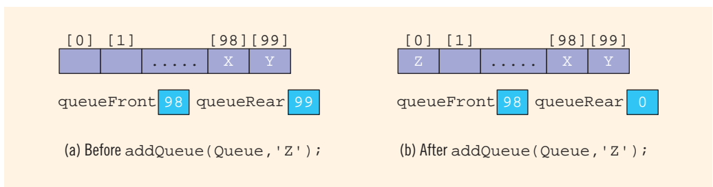
FIGURE 19-31 Queue before and after the add operation
