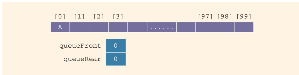
FIGURE 19-26 Queue after the first addQueue operation
