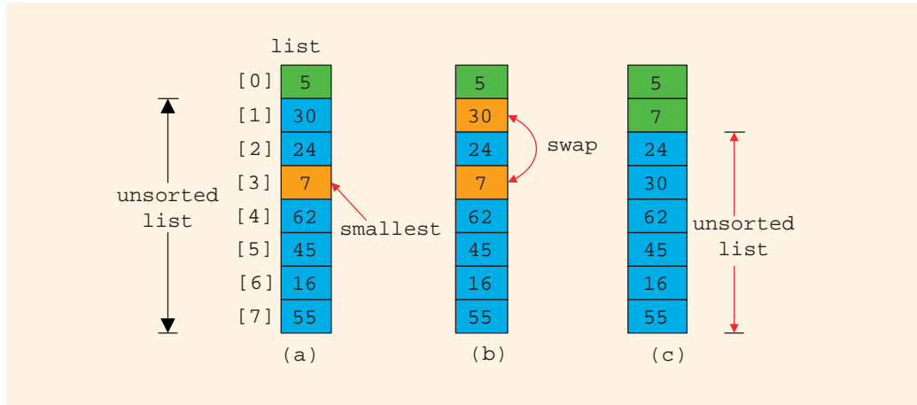
FIGURE 10-8 Elements of list during the second iteration
