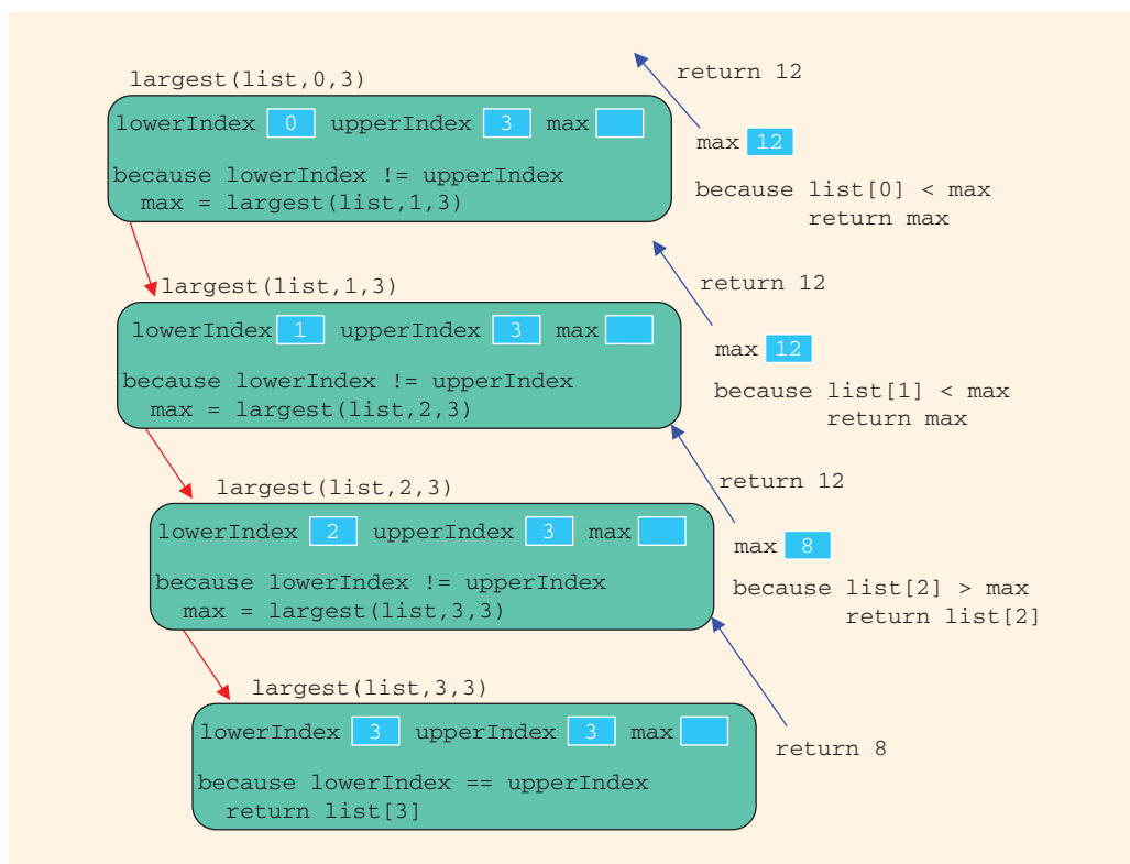
FIGURE 17-4 Execution of largest(list, 0, 3)
