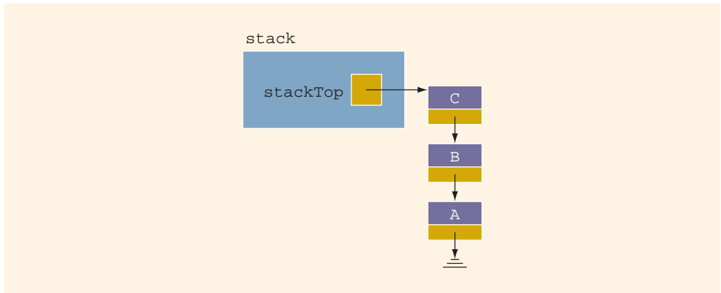
FIGURE 19-15 Stack before the pop operation
