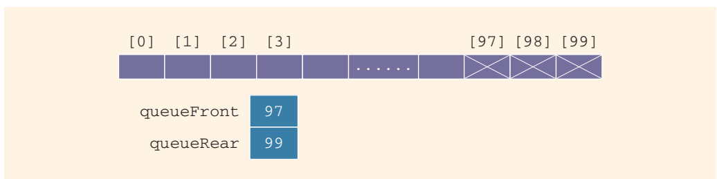
FIGURE 19-29 Queue after the sequence of operations AAADADADADADADA...
