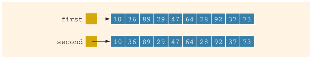
FIGURE 14-12 first and second both pointing to their own data
