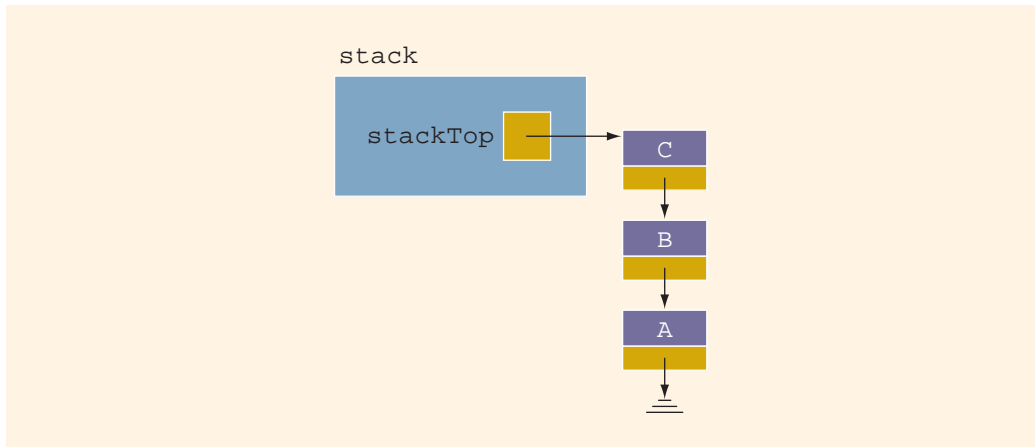
FIGURE 19-13 Stack before the push operation
