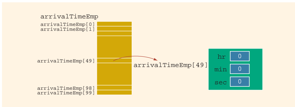
FIGURE 12-8 Array arrivalTimeEmp
