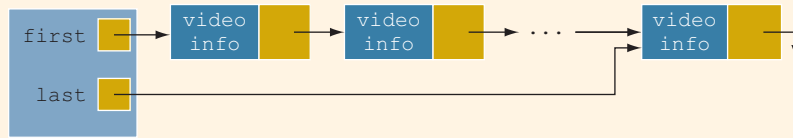
FIGURE 18-46 videoList
