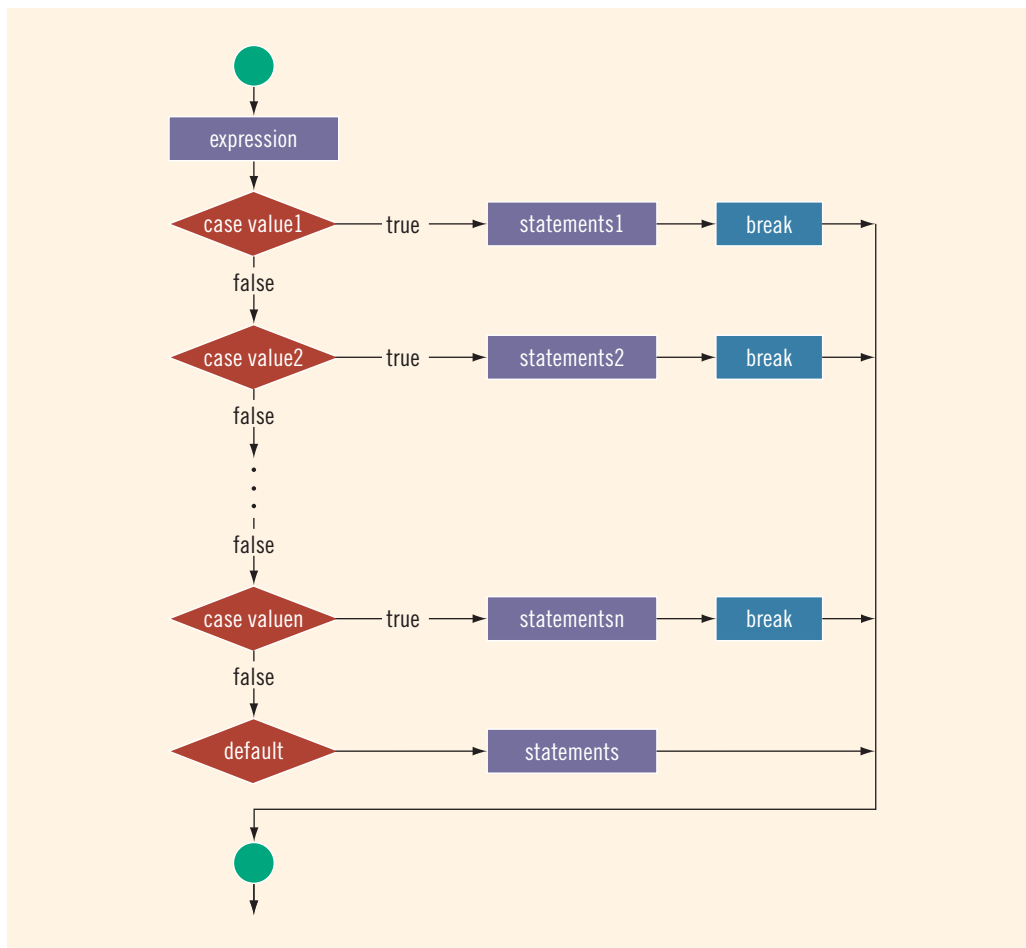
FIGURE 4-4 switch statement
