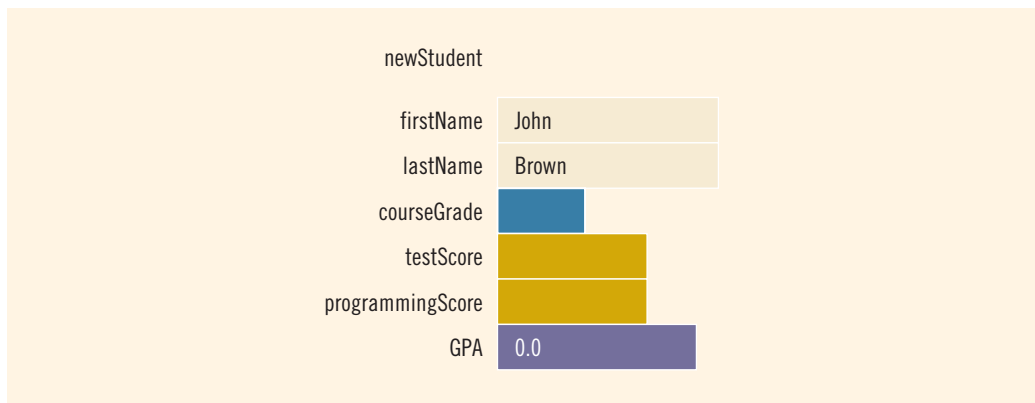
FIGURE 11-2 struct newStudent
