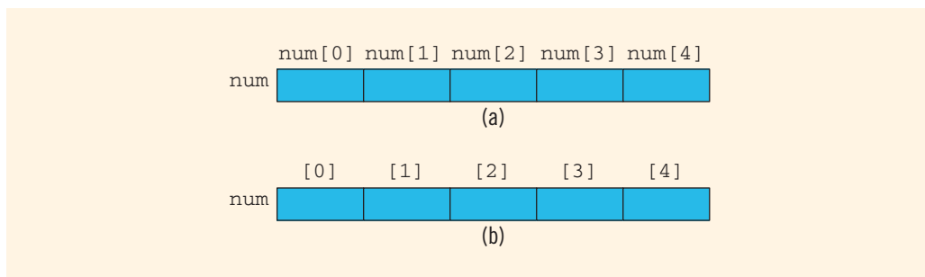
FIGURE 9-2 Array num
