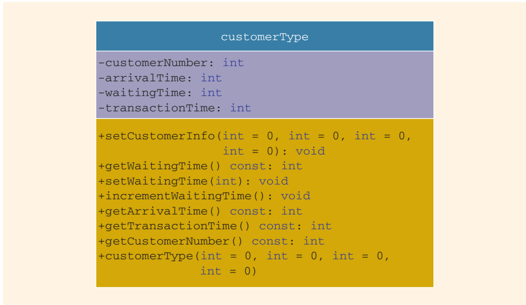
FIGURE 19-36 UML class diagram of the class customerType
