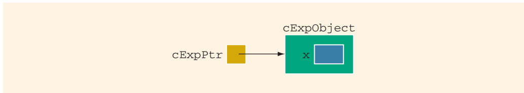
FIGURE 14-3 cExpObject and cExpPtr after the statement cExpPtr = &cExpObject; executes
