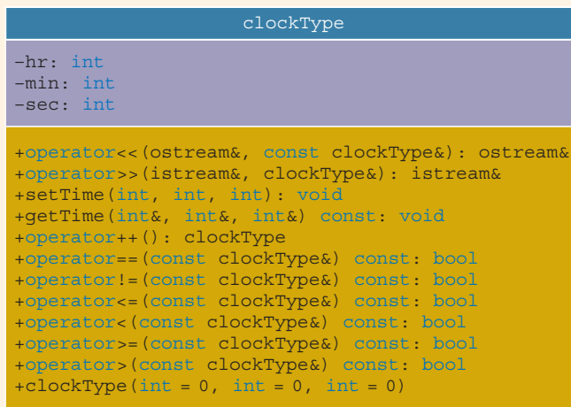
FIGURE 15-1 UML class diagram of the class clockType
