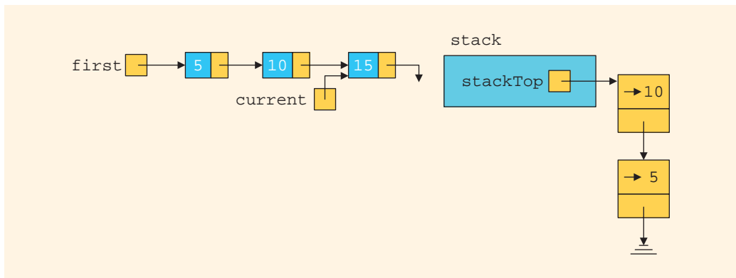
FIGURE 19-23 List and stack after the statements current = stack.top(); and stack.pop(); execute
