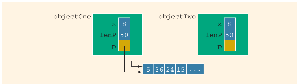
FIGURE 14-16 Objects objectOne and objectTwo after the statement objectTwo = objectOne; executes
