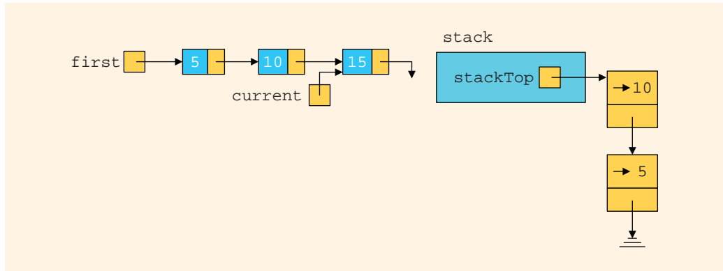
FIGURE 19-21 List and stack after the statements stack.push(current); and current = current->link; execute
