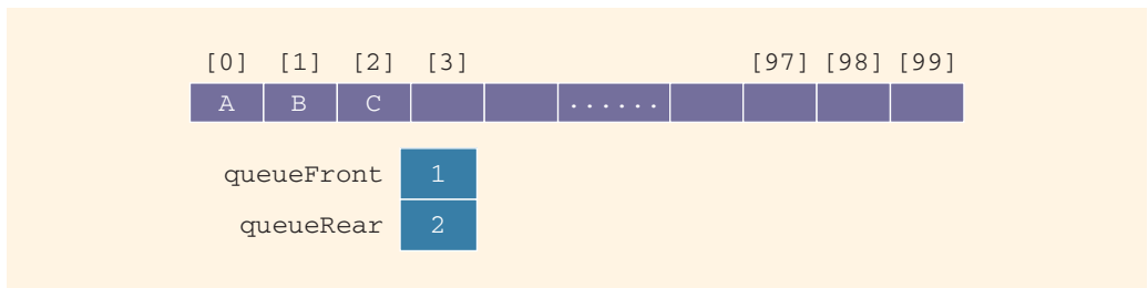
FIGURE 19-28 Queue after the deleteQueue operation
